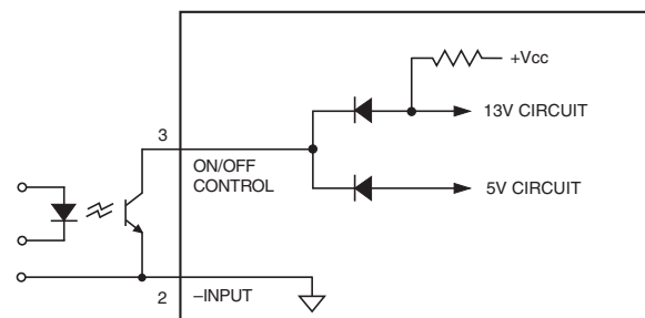
Figure 4. Driving the Positive Polarity On/Off Control Pin
