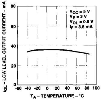
Figure 5. Low Level Output Current vs. Temperature.
