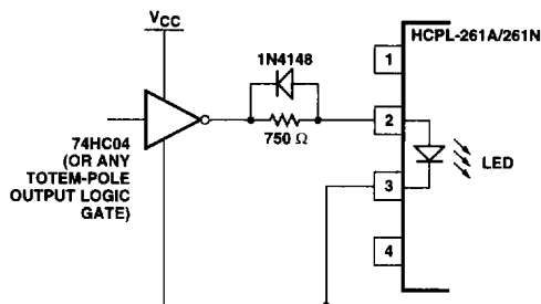
Figure 24. CMOS Gate Drive Circuit for HCPL-261A/-261N Families.
