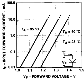
Figure 6. Typical Diode Input Forward Current Characteristic.
