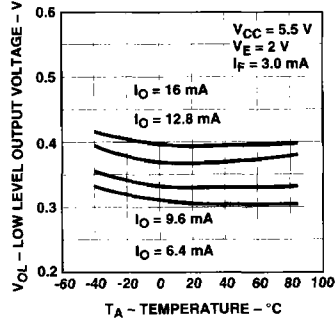
Figure 8. Typical Low Level Output Voltage vs. Temperature.
