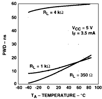
Figure 13. Typical Pulse Width Distortion vs. Temperature.
