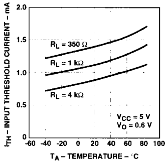
Figure 10. Typical Input Threshold Current vs. Temperature.
