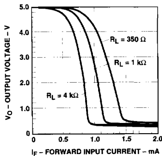
Figure 7. Typical Output Voltage vs. Forward Input Current.
