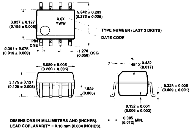
Figure 3. 8-Pin Small Outline Package Device Drawing.
