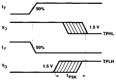
Figure 25. Illustration of Propagation Delay Skew – t_{PSK} .
