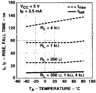
Figure 14. Typical Rise and Fall Time vs. Temperature.
