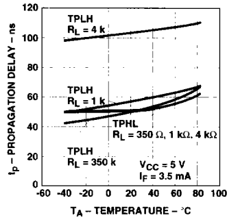
Figure 11. Typical Propagation Delay vs. Temperature.
