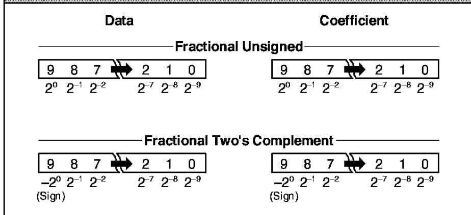
FIGURE 2A. INPUT FORMATS
