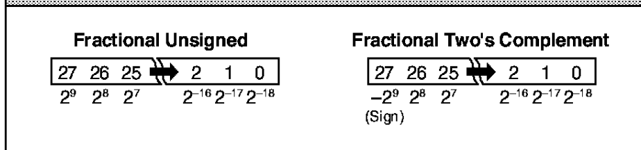
FIGURE 2B. OUTPUT FORMATS
