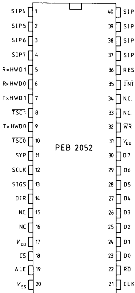
P-DIP
