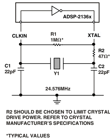
Figure 9. 333 MHz Operation (Fundamental Mode Crystal)
