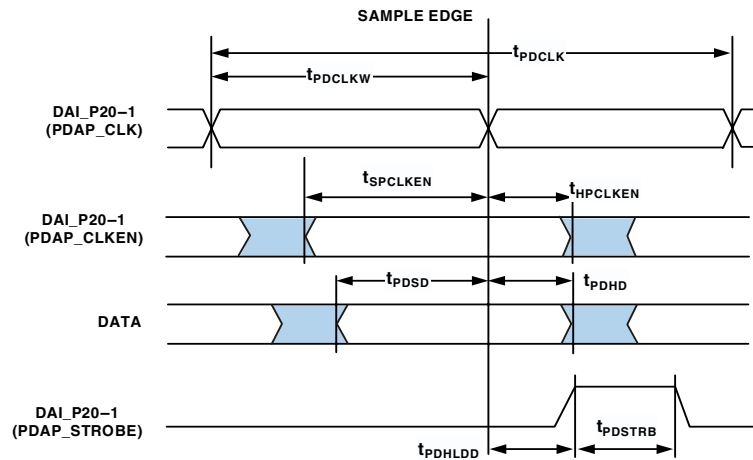
Figure 25. PDAP Timing
