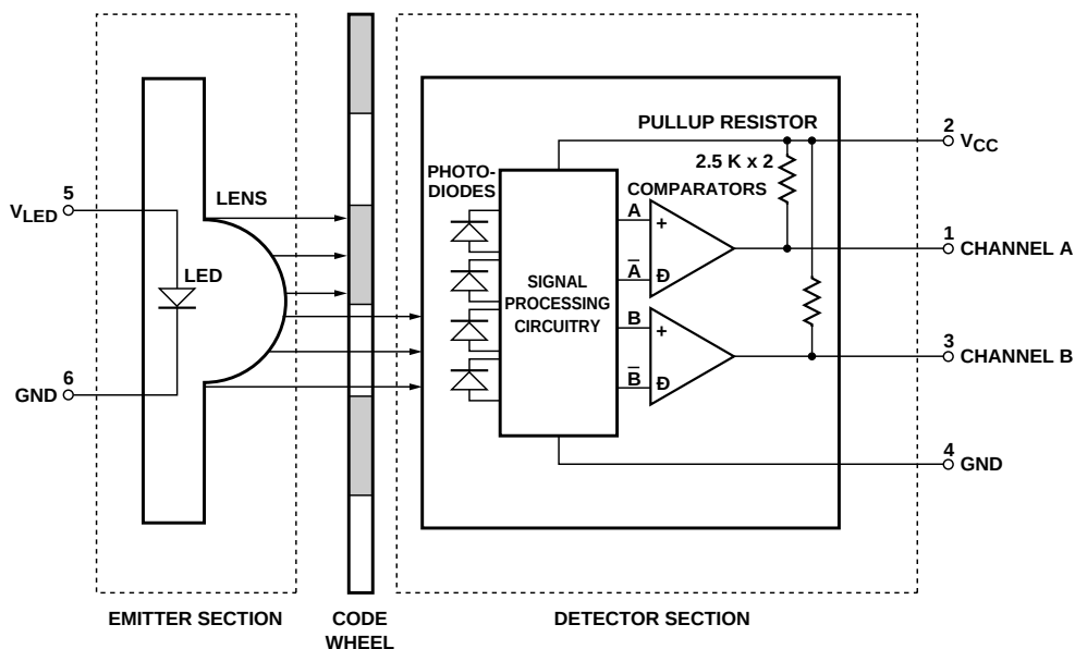
AEDS-96EX Series Block Diagram
