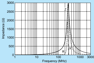
BLM15BC241SN1
