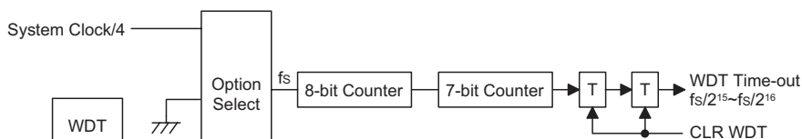
Watchdog Timer
