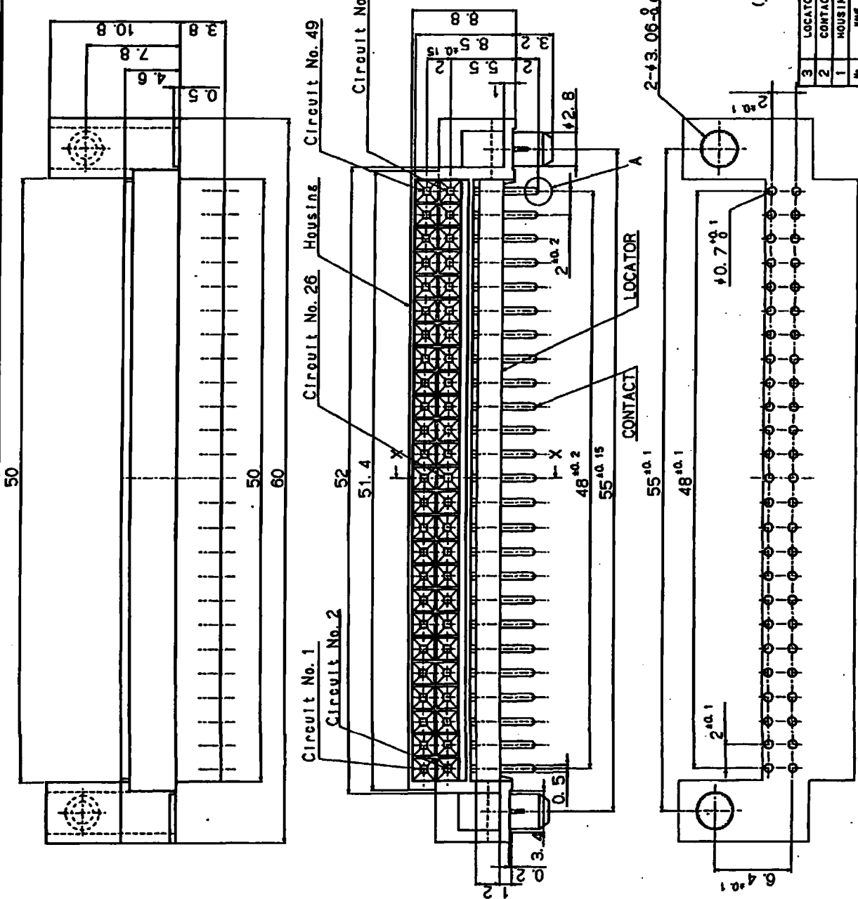
P.C. Board hole layout (Reference)
