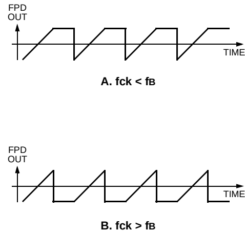
Figure 6. Frequency Detector Operation
