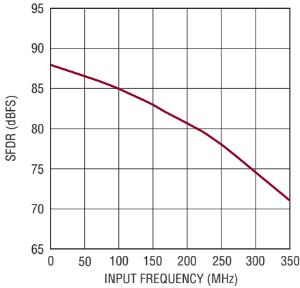
LTC2175-14: SFDR vs Input Frequency, -1dB, 2V Range, 125Mps
