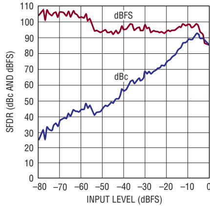
LTC2175-14: SFDR vs Input Level, f_{IN} = 70\text{MHz} , 2V Range, 125Mps
