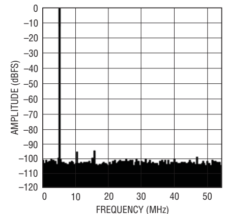
LTC2174-14: 8k Point FFT, f_{IN} = 5\text{MHz} , -1dBFS, 105Mps
