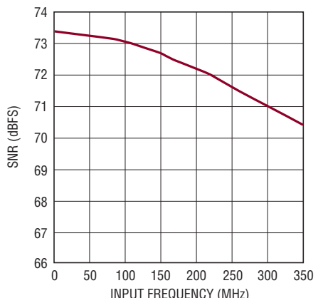
LTC2175-14: SNR vs Input Frequency, -1dB, 2V Range, 125Mps
