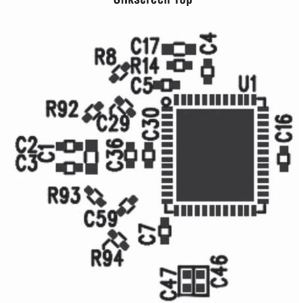
Silkscreen Top
