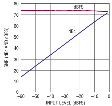
LTC2175-14: SNR vs Input Level, f_{IN} = 70\text{MHz} , 2V Range, 125Mps
