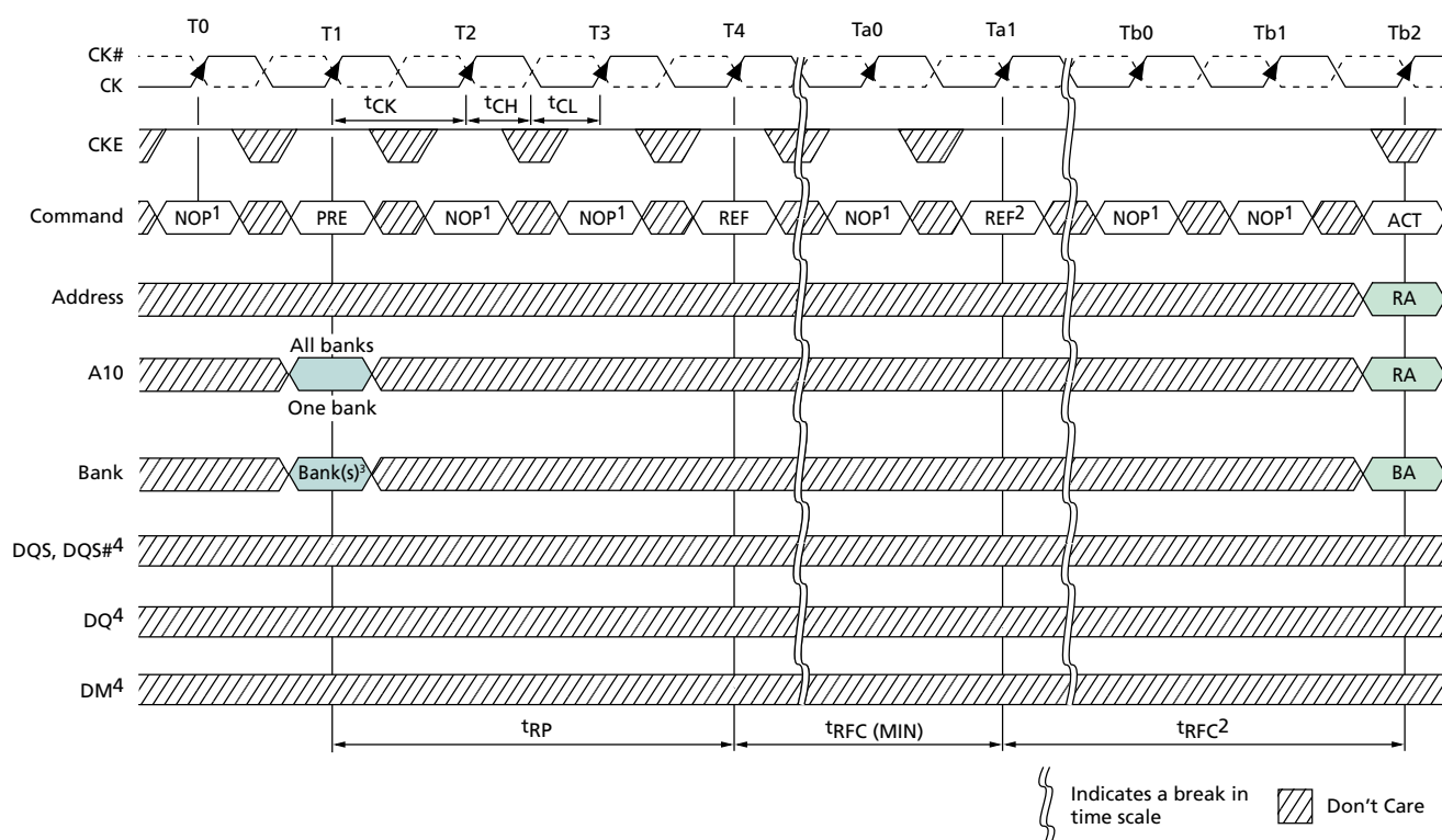
Figure 66: Refresh Mode
