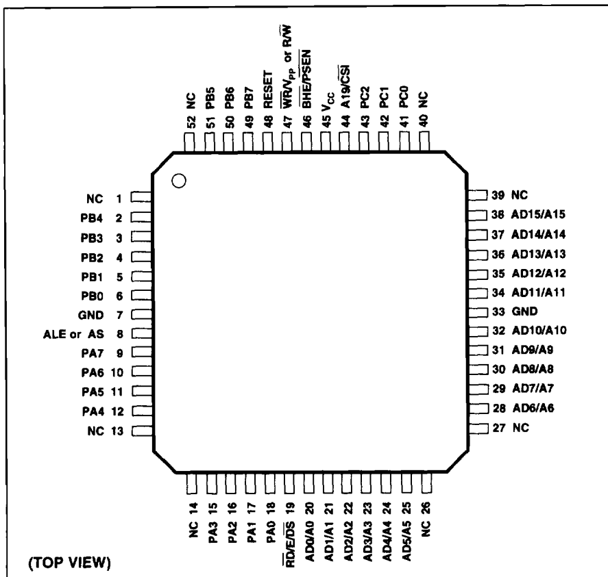
Figure 50. Drawing Q2 – 52 Pin PQFP (Package Type Q)
