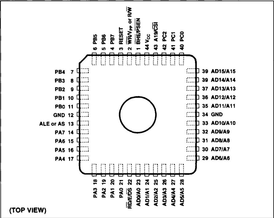
Figure 48. Drawing L4 – 44 Pin Ceramic Leaded Chip Carrier (CLDCC) with Window (Package Type L) OR Drawing J2 – 44 Pin Plastic Leaded Chip Carrier (PLDCC) without Window (Package Type J)
