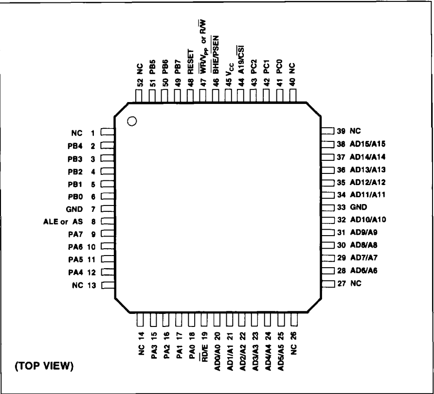
Figure 43. Drawing Q2 – 52 Pin PQFP (Package Type Q)
