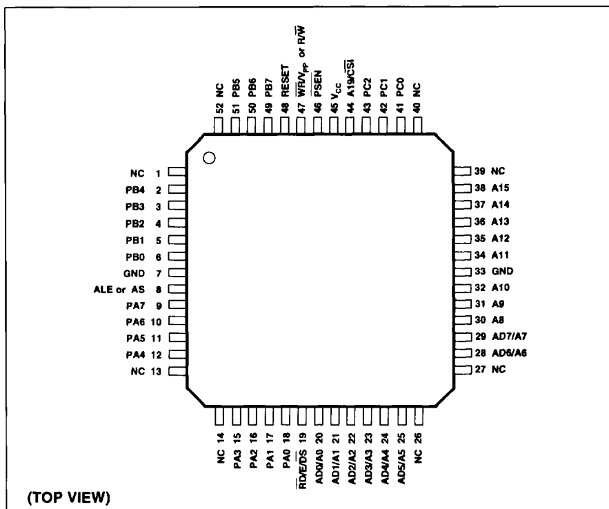
Figure 66. Drawing Q2 – 52 Pin PQFP (Package Type Q)
