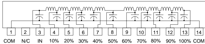
SIP5 Style Schematic
