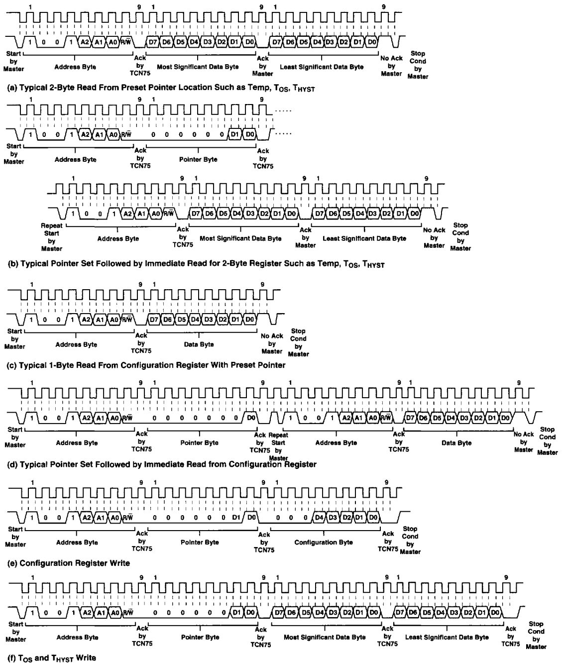
Figure 2. Timing Diagrams
