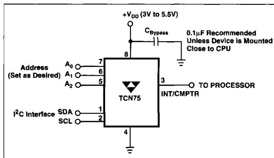
Figure 1. Typical Application
