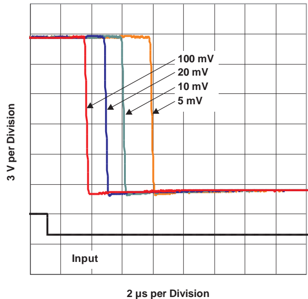
Response Time ( t_{PLH} ) for Various Input Overdrives ( V_{CC} = 15\text{ V} )
