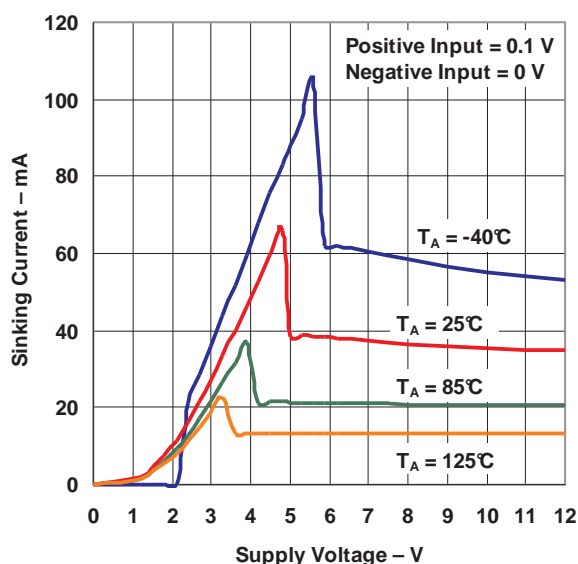
OUTPUT SINKING CURRENT vs SUPPLY VOLTAGE
