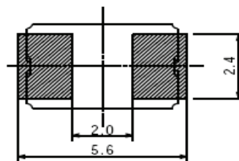
Example of a Terminal Land Pattern
