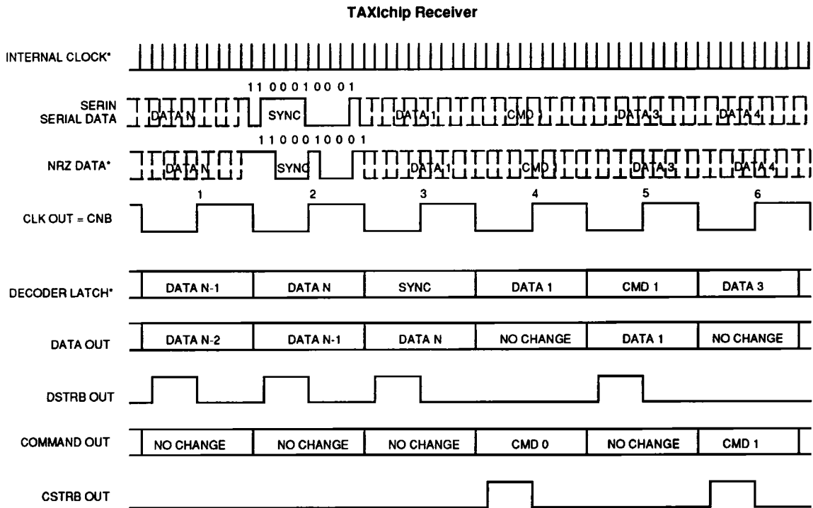
TAXIchip Receiver Timing (8-Bit Local Mode)
