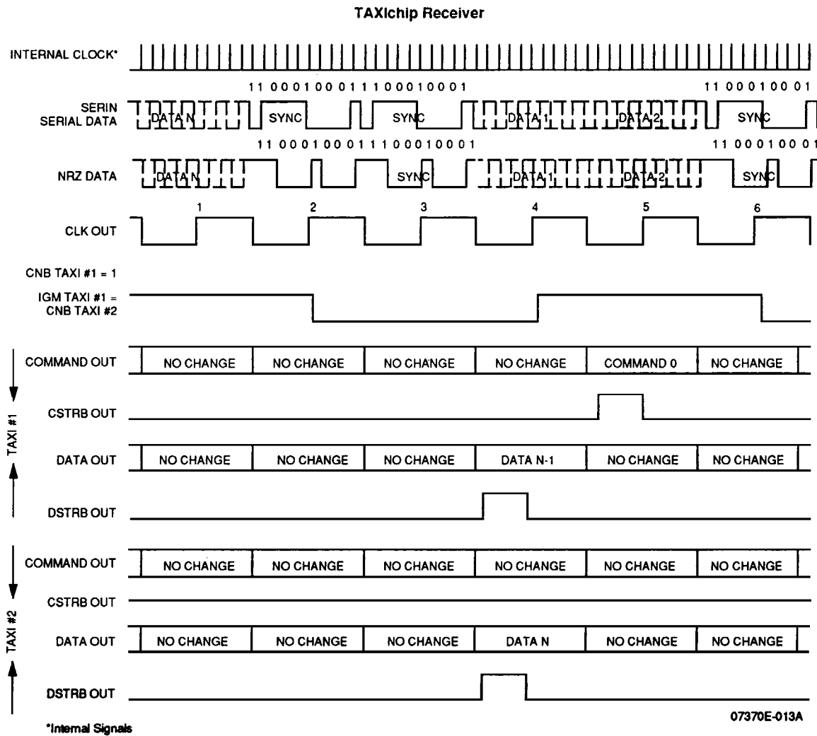
TAXIchip Receiver Timing (8-Bit Cascade Mode)
