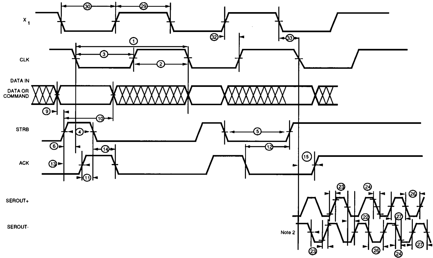
Am7968 TAXIchip Transmitter AC
