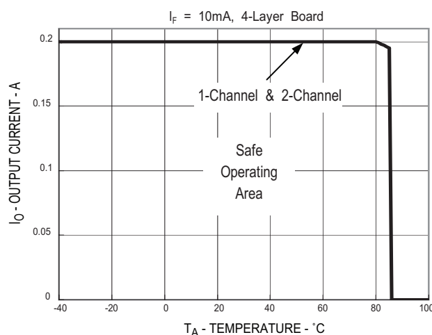
Figure 4. Maximum Output Current Rating vs Ambient Temperature (ASSR-1228-002E)
