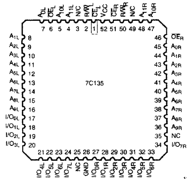
PLCC Top View
