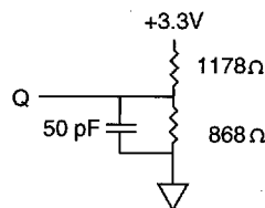
Figure 4 OUTPUT LOAD EQUIVALENT
