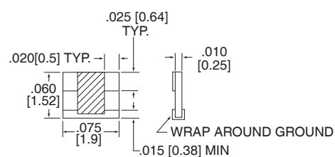
PCAAF (WRAP AROUND ALL TERMINALS)
