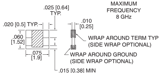
PCAAF (WRAP AROUND ALL TERMINALS)
