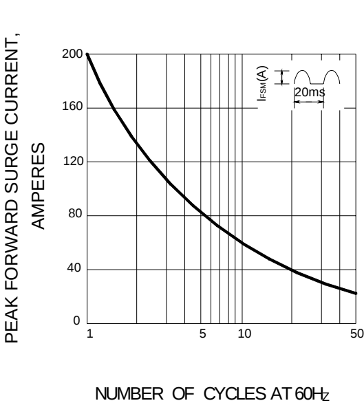
FIG.1 – PEAK FORWARD SURGE CURRENT
