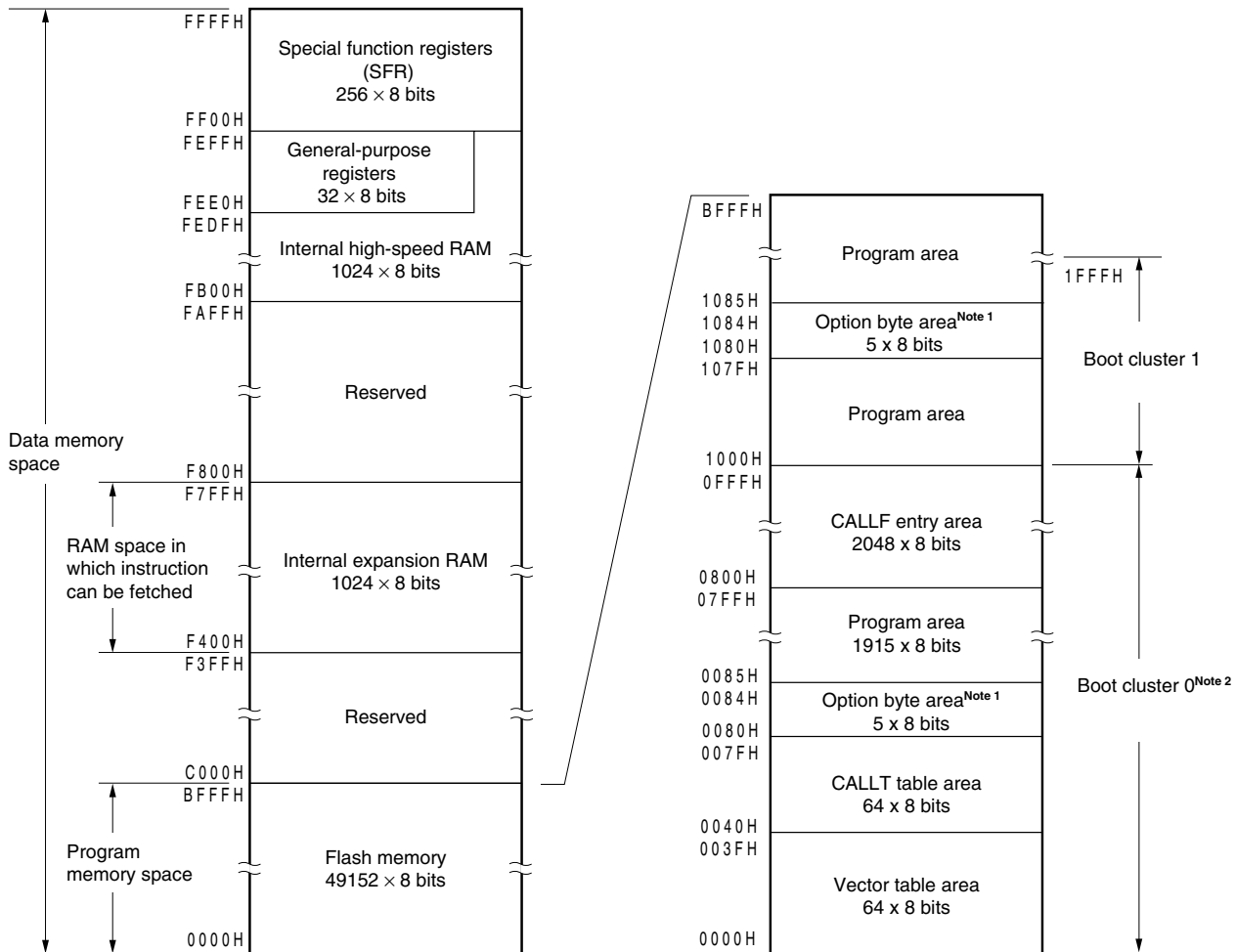
Figure 3-5. Memory Map ( \mu PD78F0514)
