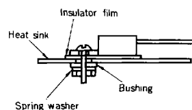
Mounting instruction
