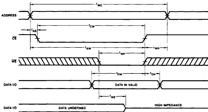
Write Cycle No. 2 ( \overline{CS} Controlled)
