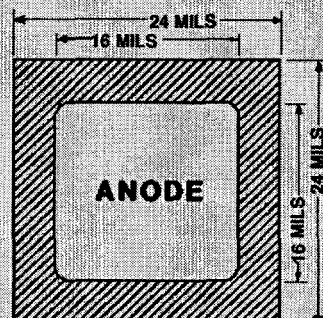
BACKSIDE IS CATHODE FIGURE 1
