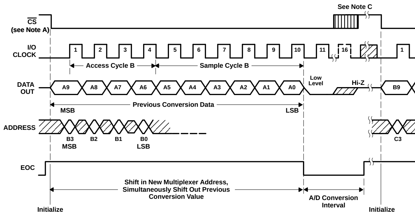
Figure 11. Timing for 11- to 16-Clock Transfer Using \overline{\text{CS}} (Serial Transfer Interval Shorter Than Conversion)
