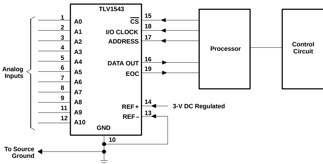
Figure 16. Serial Interface
