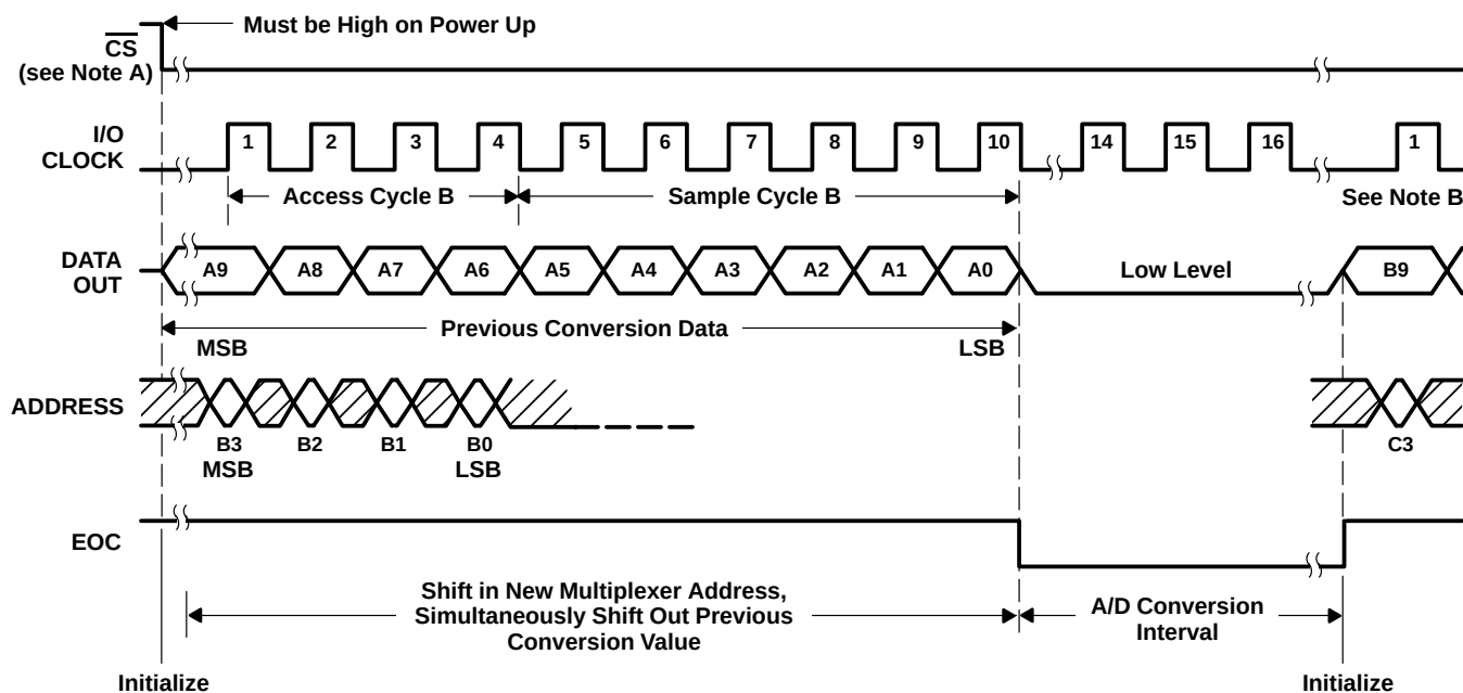
Figure 12. Timing for 16-Clock Transfer Not Using \overline{\text{CS}} (Serial Transfer Interval Shorter Than Conversion)
