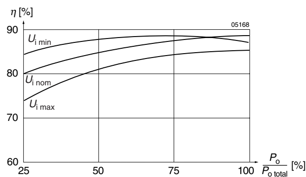
Fig. 19 Efficiency versus input voltage and load. Typical values 110 IMY 15-12-12-7
