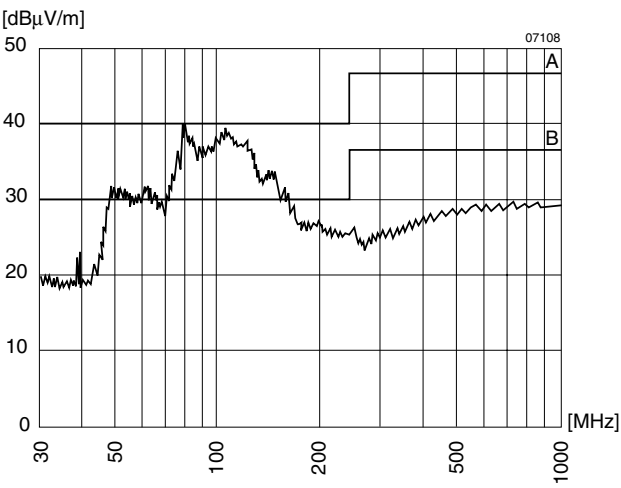
Fig. 24 Typical radio frequency-interference voltage at U_{i\text{ nom}} , I_{o\text{ nom}} , measured with an antenna (distance 10 m). Output leads 1 m, twisted.
