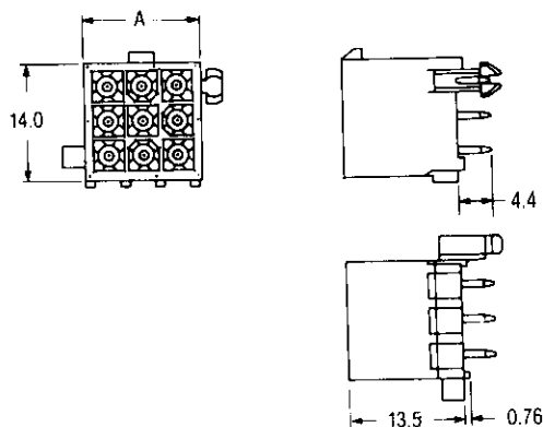
9, 12 and 15 Circuits
