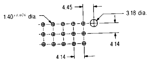
9, 12 and 15 Circuits
