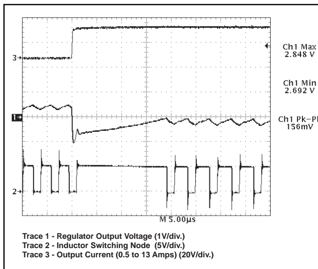
Figure 8: CS-5155 demonstration board response to 13A load turn on (output set for 2.8V). Upon completing a normal off time, the V^{2TM} control loop immediately connects the inductor to the input voltage, providing 100% duty cycle. Regulation is achieved in less than 20µs.
