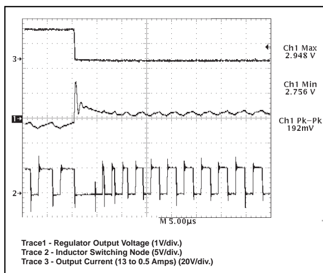
Figure 9: CS-5155 demonstration board response to 13A load turn off (output set for 2.8V). V^{2TM} control topology immediately connects inductor to ground, providing 0% duty cycle. Regulation is achieved in less than 10µs.
