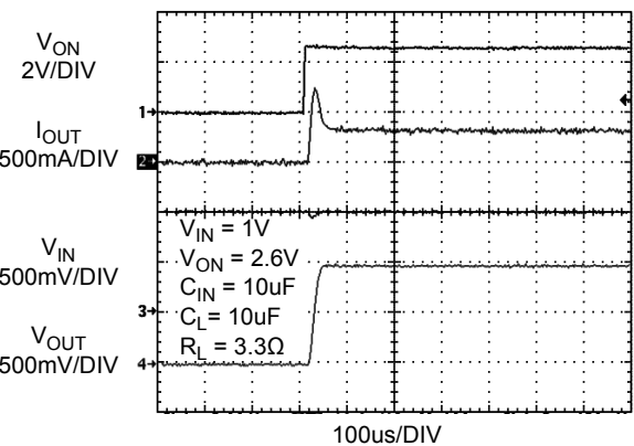
Figure 11. FPF1015 / 16 Turn ON response
