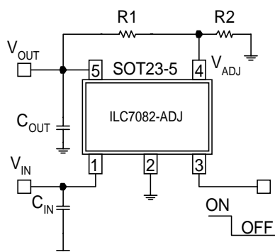
Fig. 3: Application circuit for adjustable output voltage
