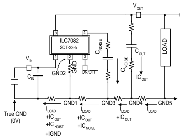
Figure 7: Effects of poor circuit layout
