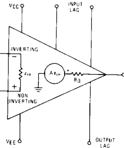
FIGURE 6 - TEST CIRCUIT
