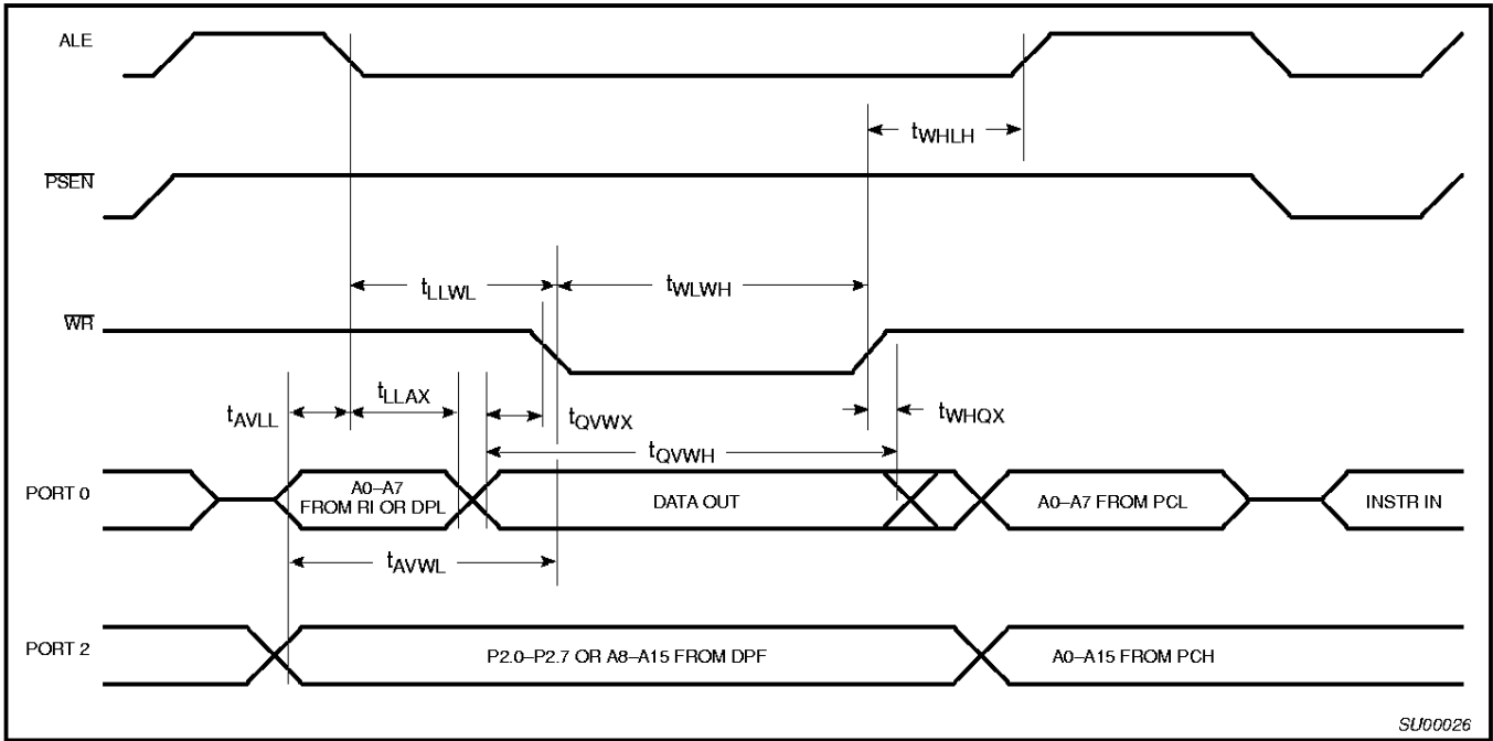
Figure 11. External Data Memory Write Cycle
