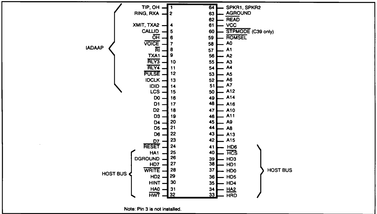
Figure 4. Parallel Pinout
