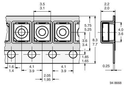
Figure 12. Tape Dimensions in mm for PLCC-2
