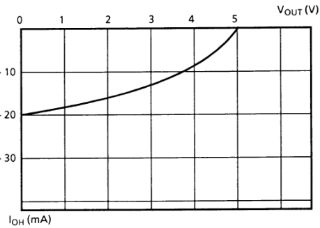
Figure 6 (5) VOUT – IOH TYPICAL CURVE
