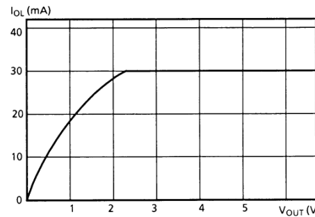
Figure 6 (4) VOUT – IOL TYPICAL CURVE
