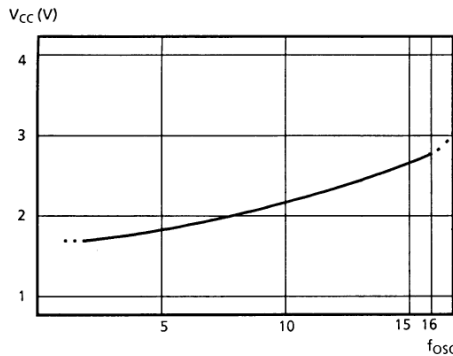
Figure 6 (1) VCC – fOSC TYPICAL CURVE
