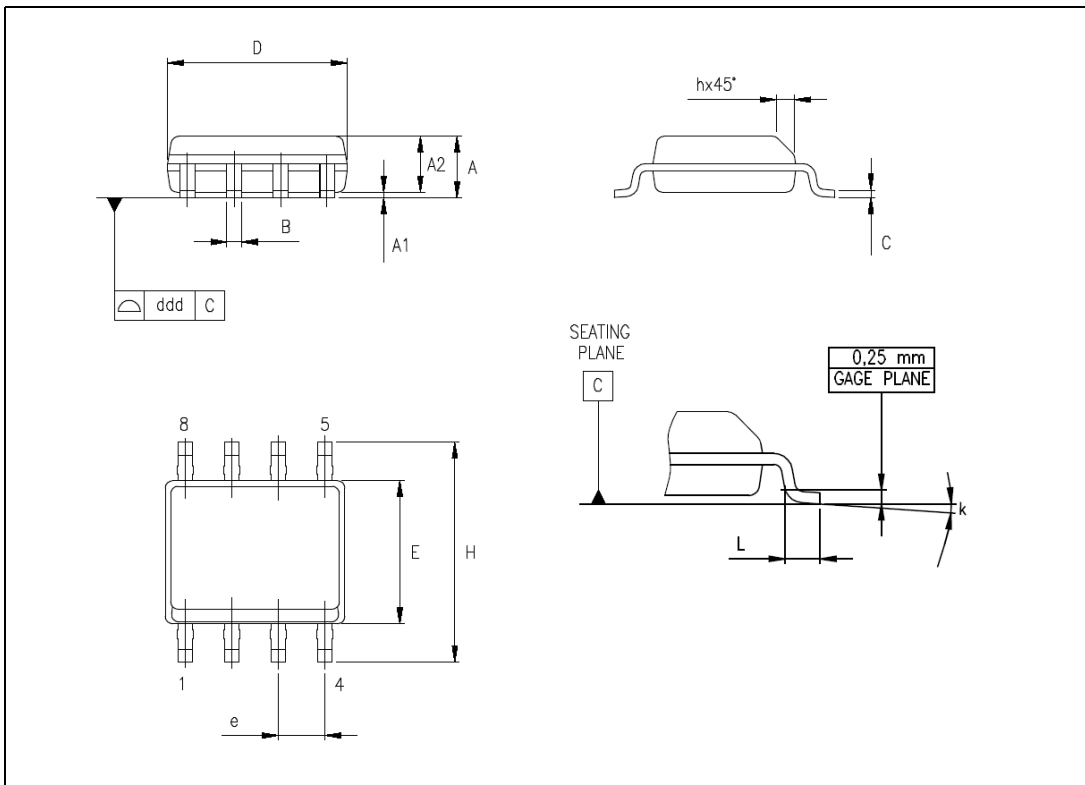
Figure 16. Package Dimensions
