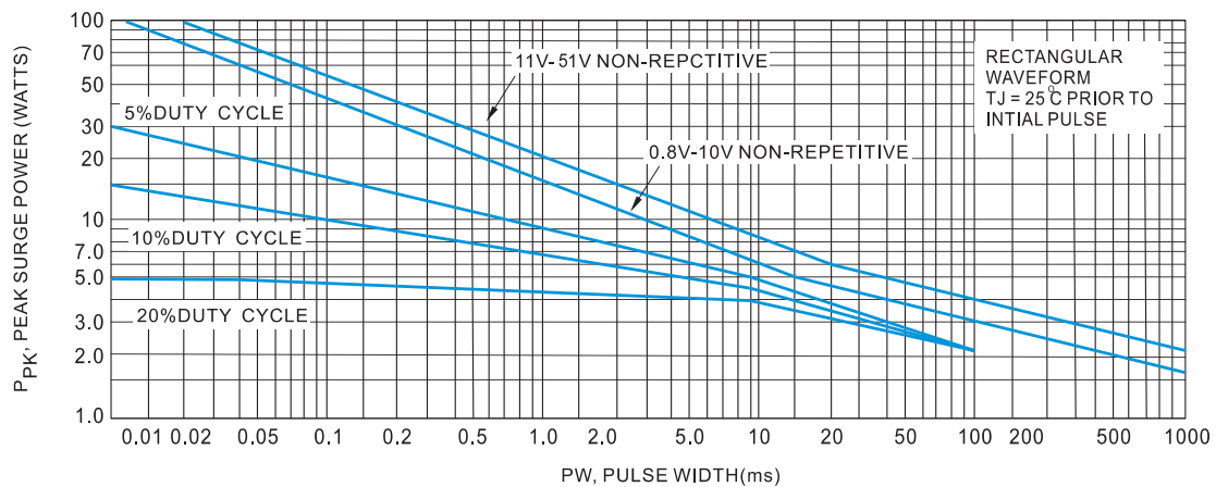
FIGURE.5 MAXIMUM SURGE POWER
