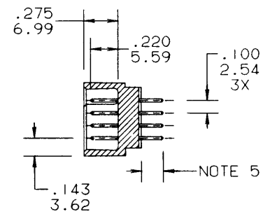
SECTION X-X
