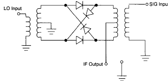
Figure 4. Typical Mixer Circuits
