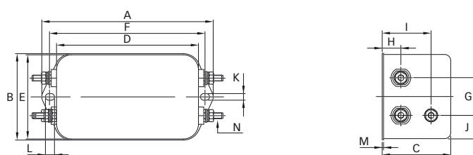
Connection style -08, 25 and 36A types
