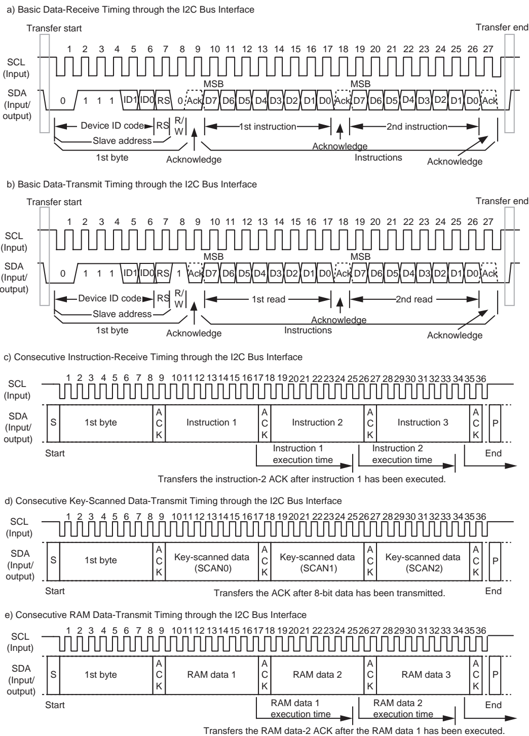
Figure 23 I 2 C Bus Interface Timing Sequence
