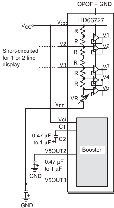
b) Triple boosting
