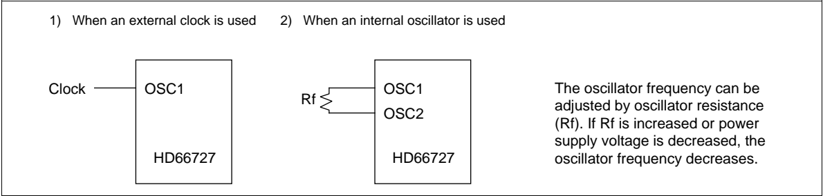
Figure 31 Oscillator Circuit
