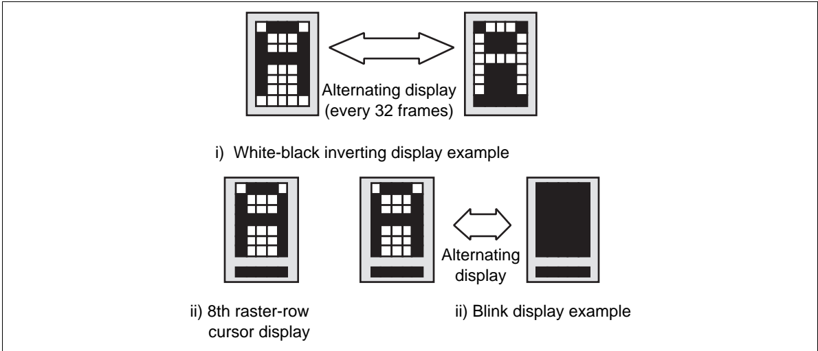
Figure 11 Cursor Control Examples
