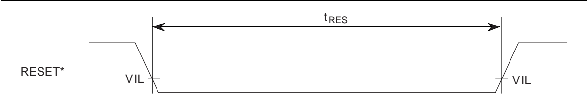
Figure 60 Reset Timing
