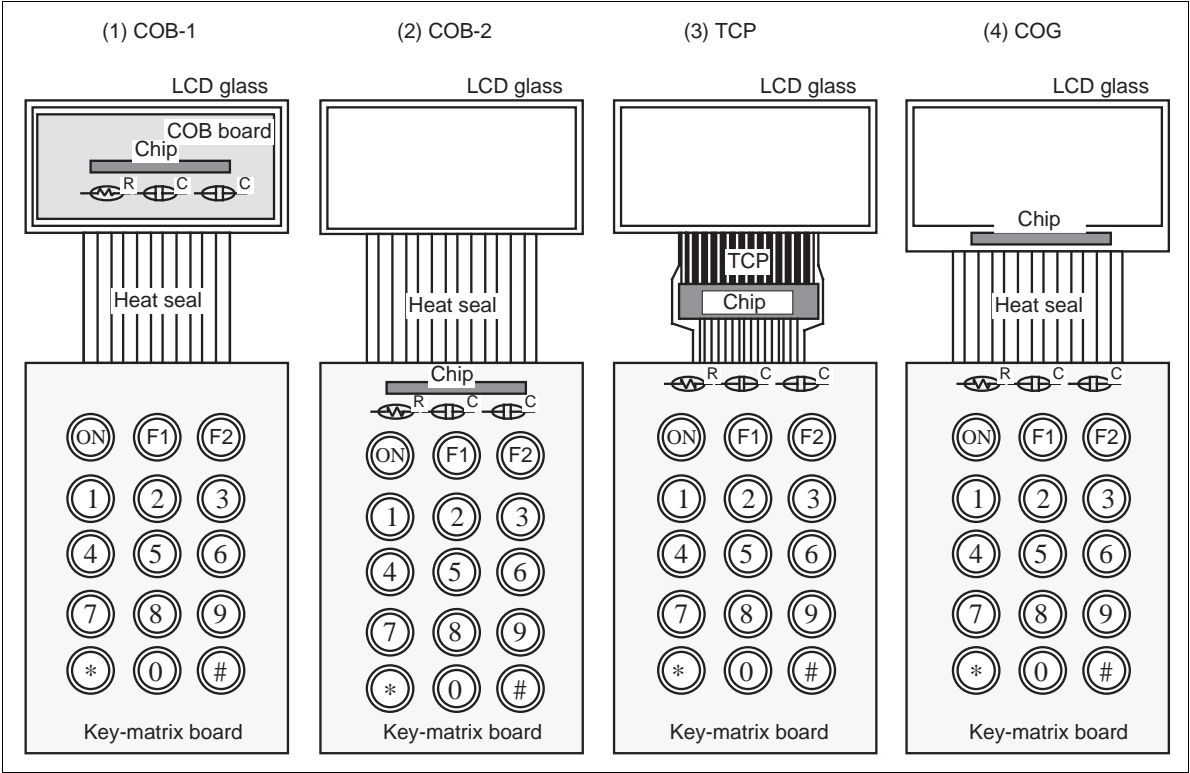
Figure 1 HD66727 Mounting Variations
