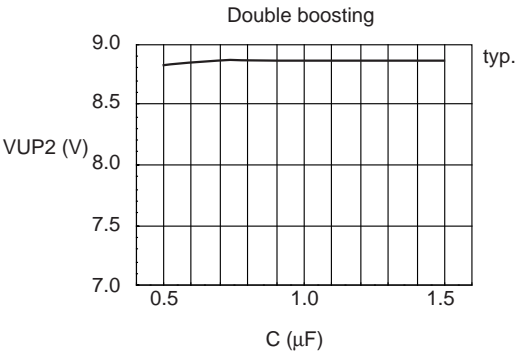
Figure 55 Booster (cont)
