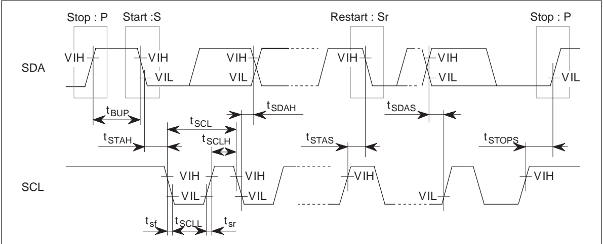
Figure 59 I 2 C Bus Interface Timing
