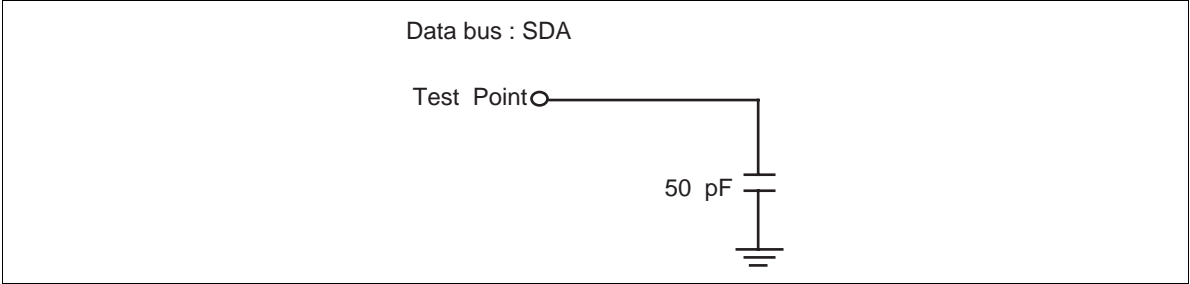
Figure 56 Load Circuit
