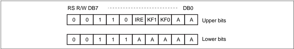
Figure 20 DDRAM Address Set Instruction
