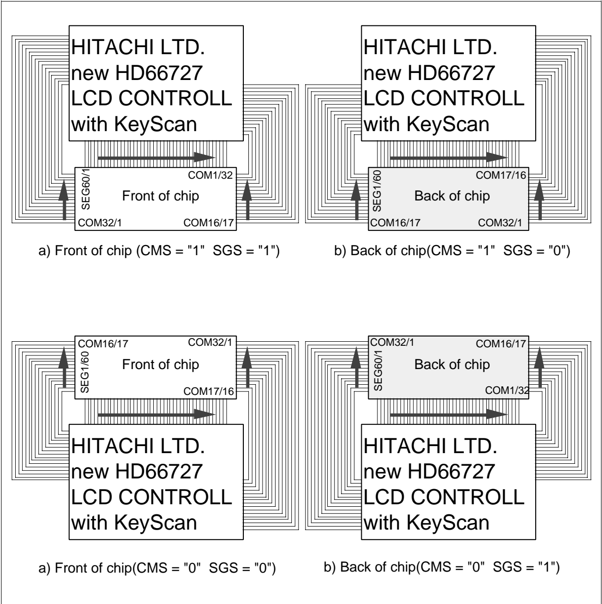
Figure 39 LCD Module Interface Examples
