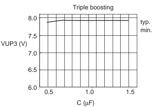
Figure 55 Booster (cont)
