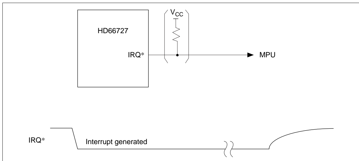
Figure 29 Interrupt Generation
