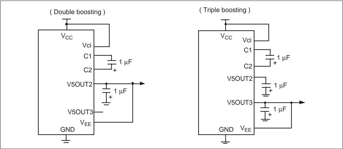
Figure 55 Booster
