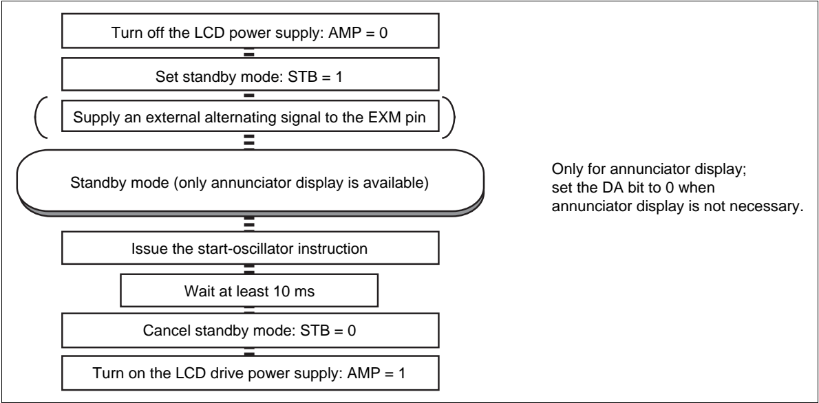
Figure 50 Procedure for Setting and Canceling Standby Mode
