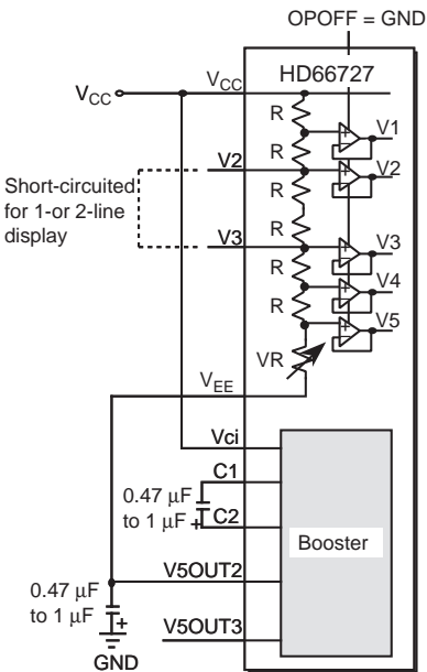
a) Double boosting
