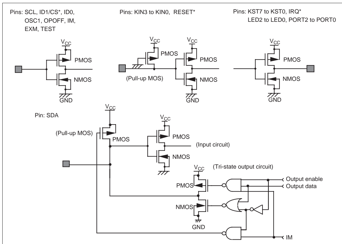
Figure 51 I/O Pin Configurations
