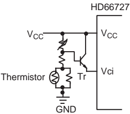
Figure 35 Temperature Compensation Circuit Example
