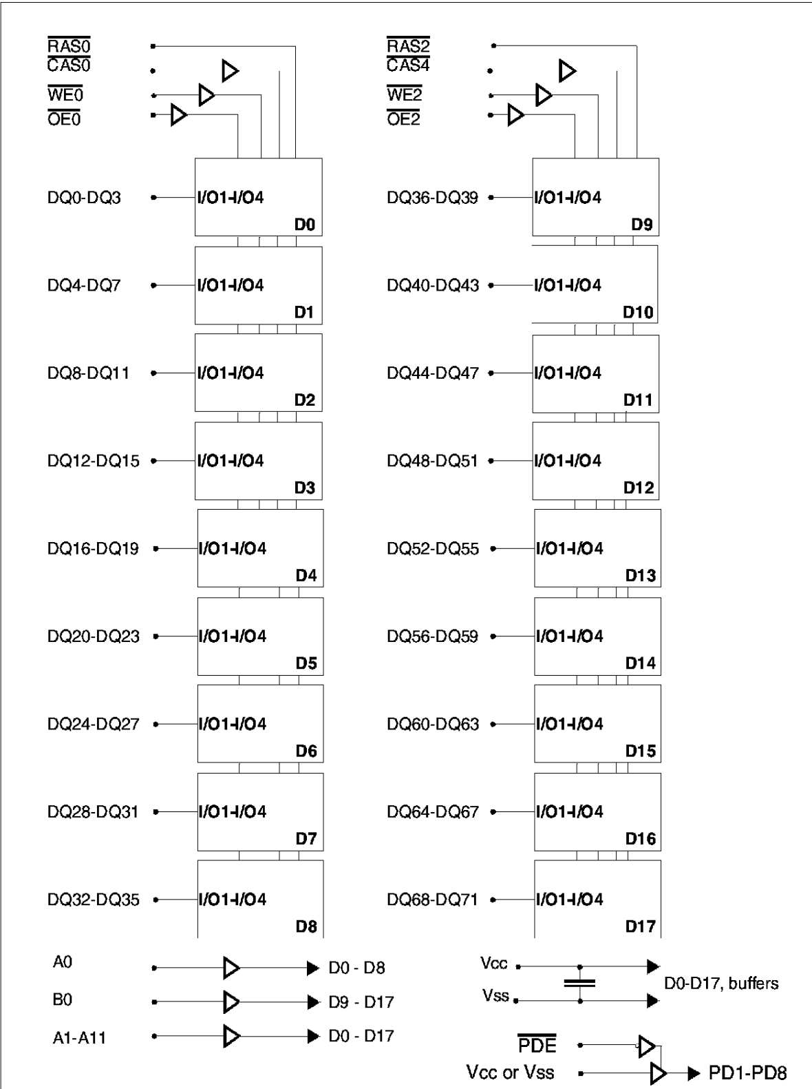
Block Diagram
