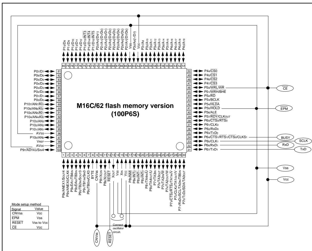
Figure 1.31.1. Pin connections for serial I/O mode (1)
