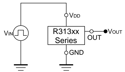
Test Circuit for Output Delay Time (CMOS Output type; pull-up is not necessary.)
