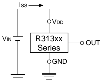
Test Circuit for Supply Current
