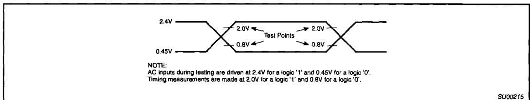
Figure 6. AC Testing Input/Output
