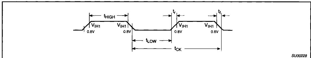
Figure 5. External Clock Drive XTAL1
