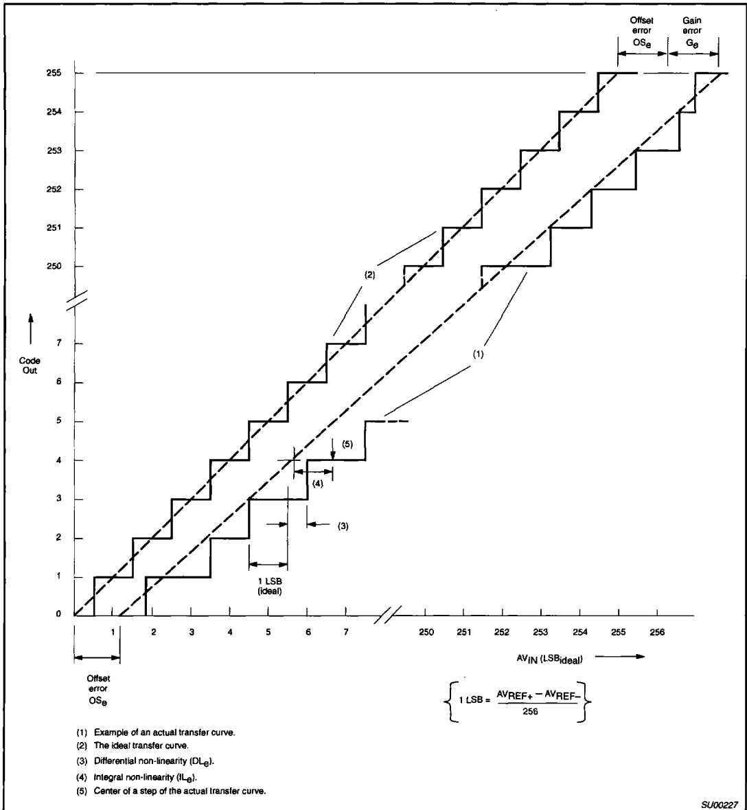
Figure 1. ADC Conversion Characteristic
