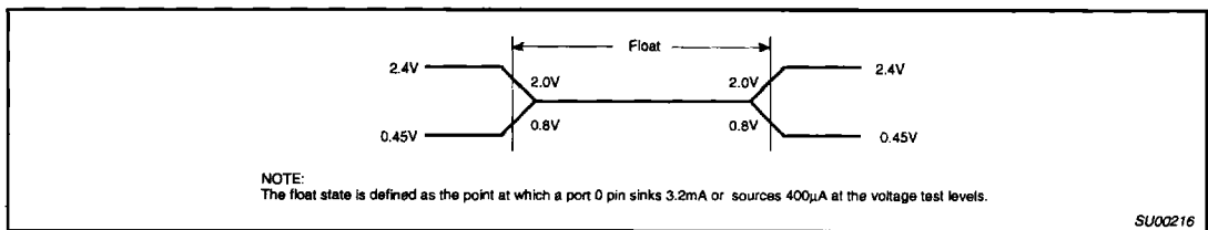
Figure 7. AC Testing Input, Float Waveform
