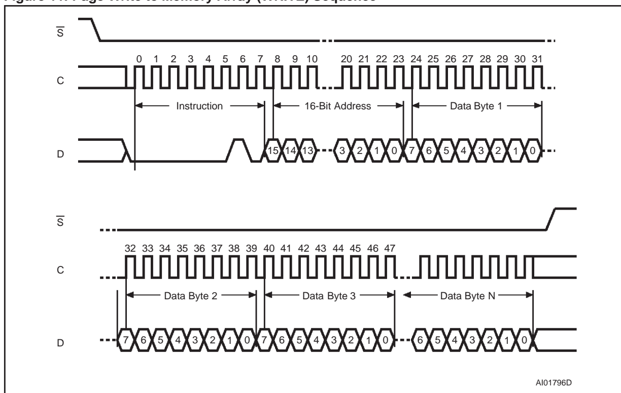
Figure 11. Page Write to Memory Array (WRITE) Sequence
