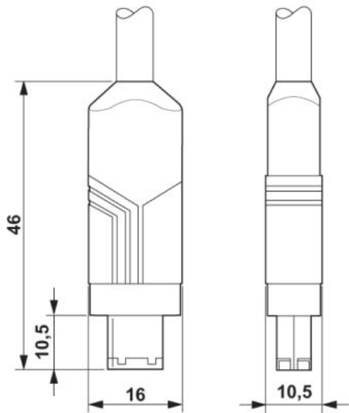
FireWire plug connector, standard
